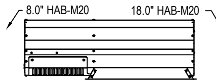
END CLEARANCES
